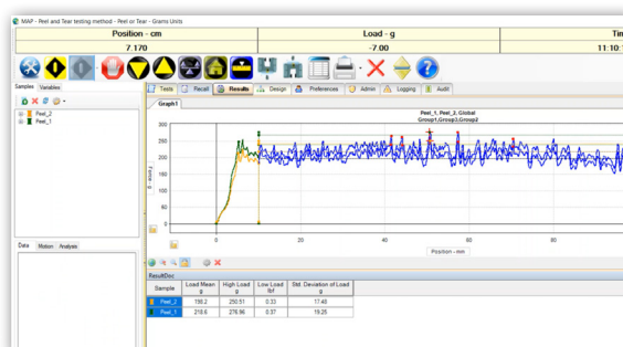
↑ Sample MAP4 Results for Peel Testing
