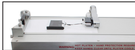
Heated Platen - Temp Range up to 204.4°C (up to 400°F)
