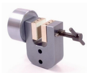
TA240k+ko with TA240k+BP pyramid jaws
