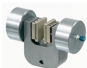
TA240k-S20+2ko with TA240k-EBP pyramid inset jaws
