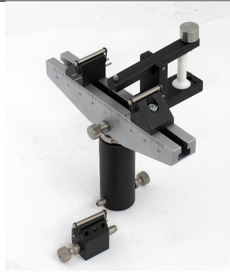
TA238-CWXD4-iTH2 holder for external Extensometer
