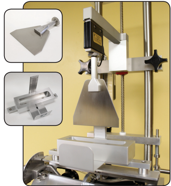
▲ Score Bend Fixture Part #202-3010
