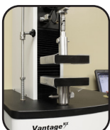
Film Blocking Fixture ASTM D3354
